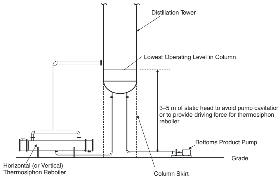
Figure 1.12 Sketch Illustrating Reasons for Elevating Distilling Column
