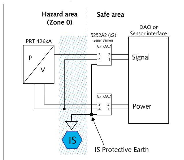
PRT 426xA with V output (3-wire)
