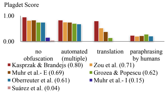
Figure 2: Results of top performing PDS in PAN-PC'10 [35]
