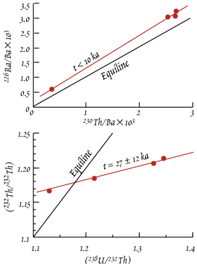
Figure 8.22. 230 Th– 238 U and 226 Ra– 230 Th mineral isochrons for the Castle Creek andesite of Mt. St. Helens. 14 C and tree ring chronology indicate this lava was erupted 1700–2200 years ago. After Volpe and Hammond (1991).
