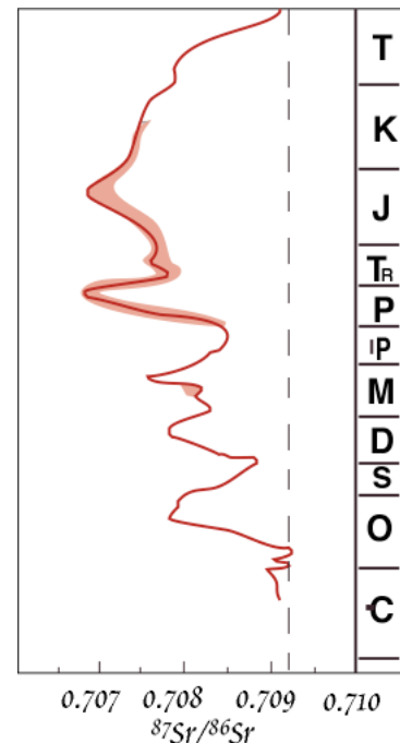
Figure 8.8. ^{87}\text{Sr}/^{86}\text{Sr} in seawater through Phanerozoic time determined from the analysis of phosphate and carbonate fossils. Dashed line shows the composition of modern seawater, grayed areas represent uncertainties.
